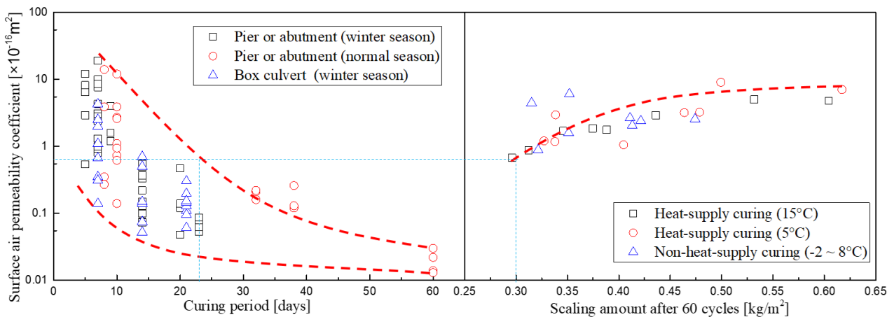
Fig. 7 – The relationship between curing period and the scaling amount after 60 cycles of freezing-thawing action
