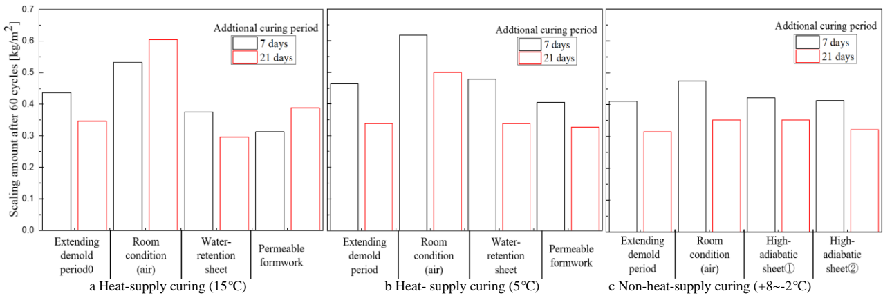
Fig. 6 – The scaling amount after 60 cycles of freezing-thawing action
