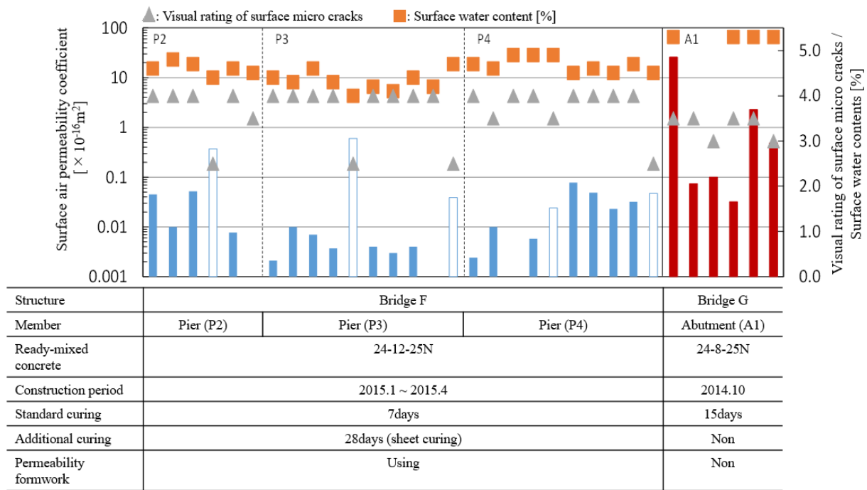
Fig. 5 – Effect of the permeability formwork on the surface air permeability of structure
