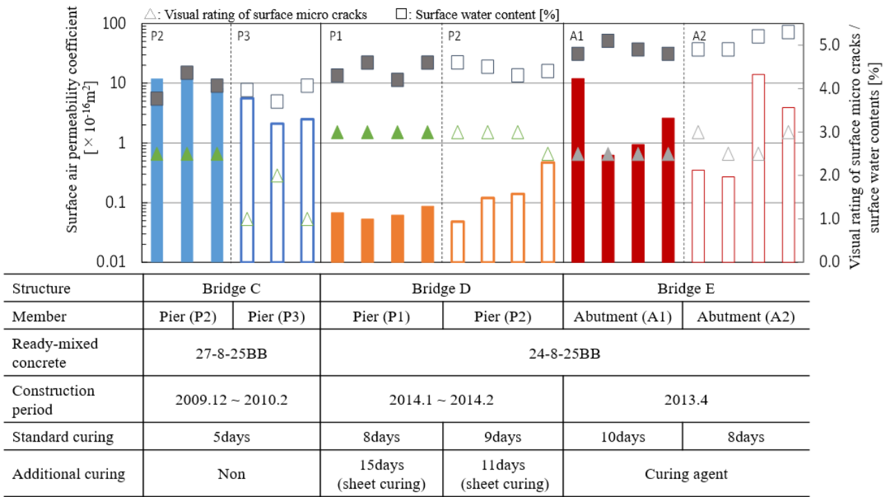
Fig. 3 – Effect of the additional curing on the surface air permeability of existing structure
