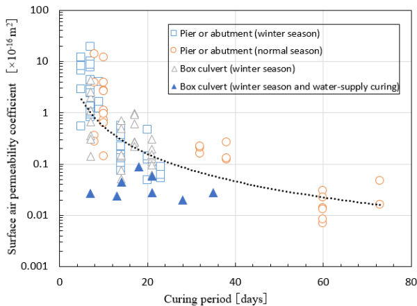
Fig. 4 – The relationship between the surface air permeability coefficient and curing period
