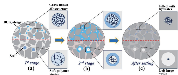
Figure 4. Schematic illustration of the internal curing mechanism of superabsorbent polymers (SAPs) in UHPC during hydration [47].
