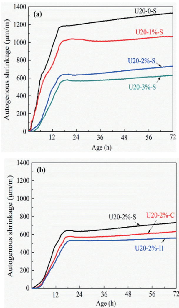
Figure 8. Influence of steel-fiber content and geometry on the development of autogenous shrinkage in UHPC. (a) Different steel-fiber volume fractions; (b) Different fiber geometries [76].
