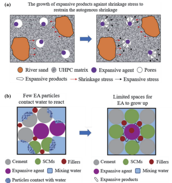
Figure 10. Schematic illustration of the compensatory expansion mechanism of expansive agents and their limitations in UHPC: (a) shrinkage compensation by expansive products; (b) restricted hydration and expansion space in dense UHPC matrix. Adapted from [90].
