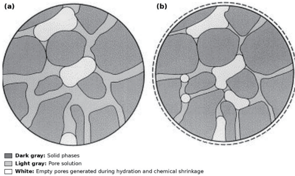
Figure 2. Schematic illustration of self-desiccation development in UHPC during hydration: (a) low degree of hydration; (b) high degree of hydration [32].
