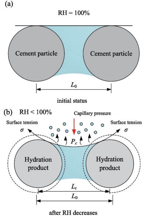
Figure 3. Schematic illustration of capillary pressure development during self-desiccation in UHPC [35].
