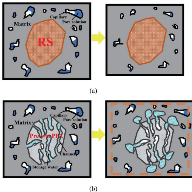
Figure 5. Schematic illustration of water release behavior in porous aggregates during hydration: (a) conventional aggregate (RS) without water release capacity; (b) pre-wetted porous fine aggregate (PFA) providing internal curing through gradual water desorption via interconnected pore channels [61].
