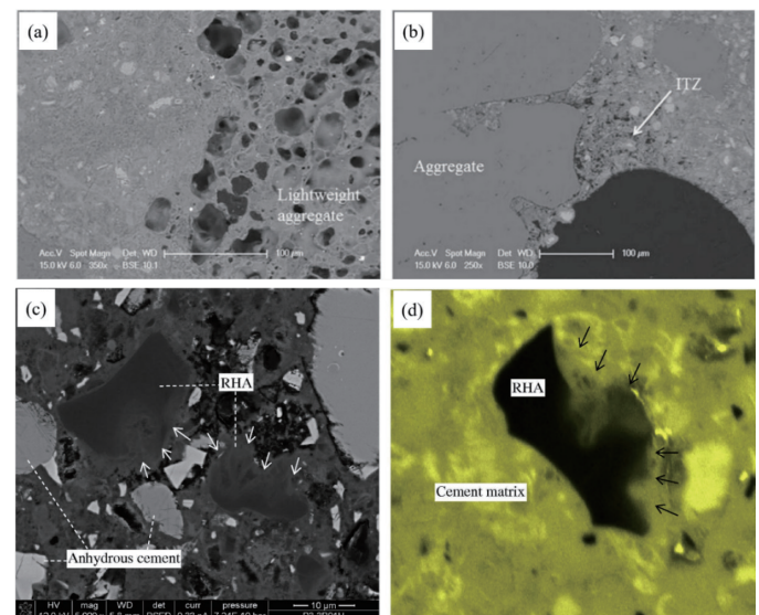
Figure 6. Representative interfacial characteristics of porous aggregates and porous powders in cementitious matrices: (a, b) lightweight aggregate (LWA) and its interfacial transition zone (ITZ); (c, d) rice husk ash (RHA) particles embedded within the cementitious matrix [58, 62].
