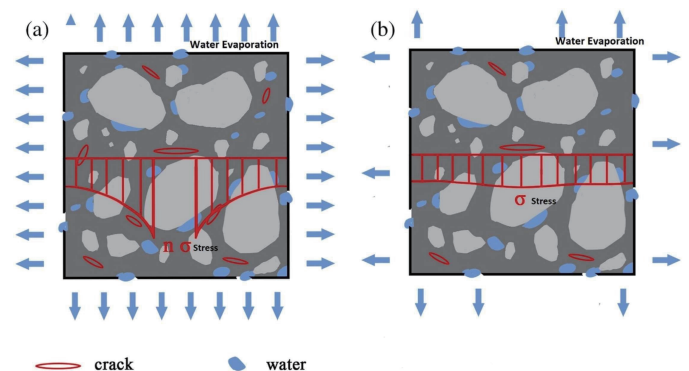
Figure 7. Schematic illustration of fiber-bridging and stress-redistribution mechanisms for controlling shrinkage-induced cracking: (a) plain matrix and (b) fiber-reinforced matrix.
