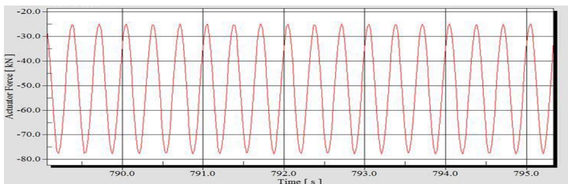
Fig. 6 – Cyclic loading at 3 Hz
