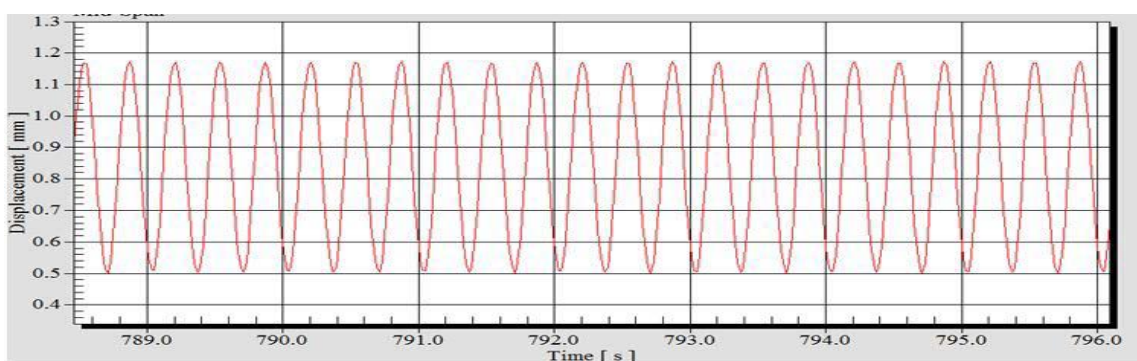
Fig. 7 – Deflection under cyclic loading
