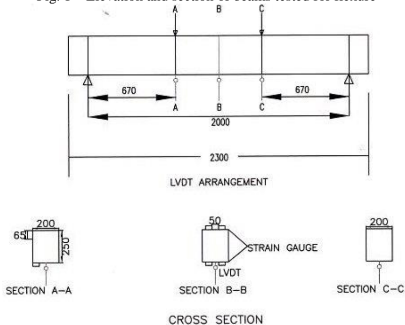
Fig. 2 – Testing setup along with instrumentation details
