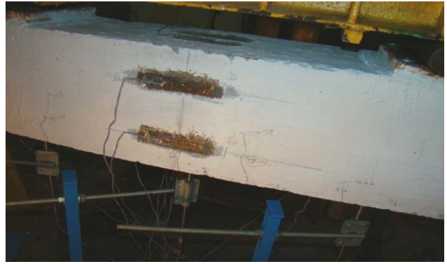
(b) final cracking at ultimate load
