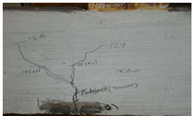
(h) final cracking at ultimate load
