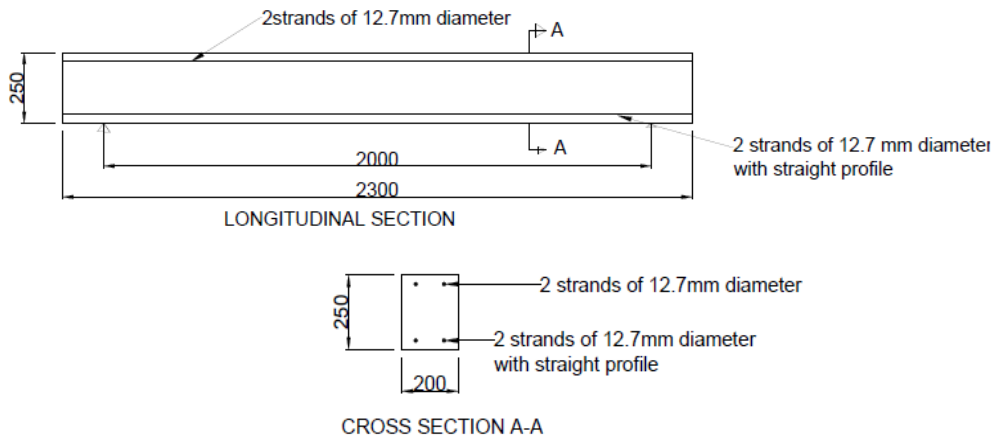
Fig. 1 – Elevation and section of beams tested for flexure
