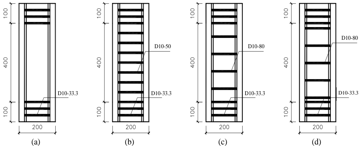
Fig. 2 – Longitudinal sections of internal confinement arrangements of specimens: (a) CS01, S04, S04c, S04d, S04e, S04f; (b) CS03a; (c) S04a; (d) S04b
