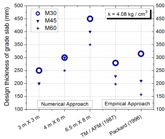
Fig. 7 – Comparison of design thickness of grade slab by empirical and numerical approaches for modulus of sub-grade reaction = 4.08 kg/cm 3
