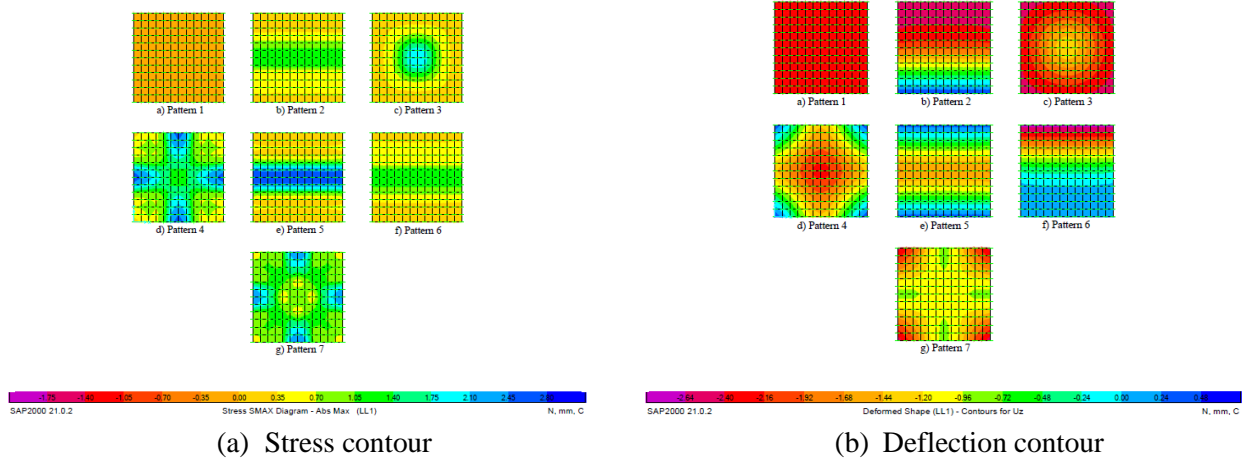
Fig. 2 – Contours for different loading patterns (modulus of sub-grade reaction of 3.00 kg/cm 3 )
