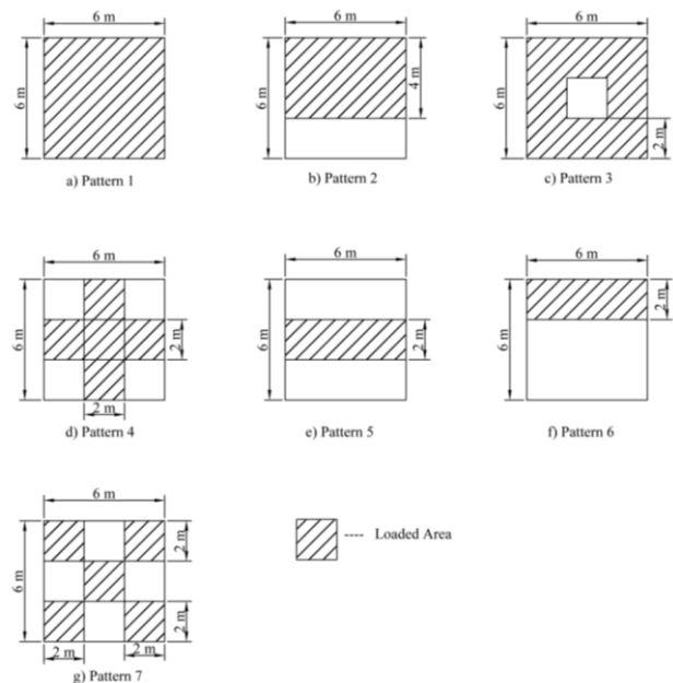
Fig.1 – Different loading patterns considered in numerical analysis of grade slab panel
