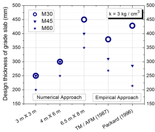
Fig. 6 – Comparison of design thickness of grade slab by empirical and numerical approaches for modulus of sub-grade reaction = 3 kg/cm 3
