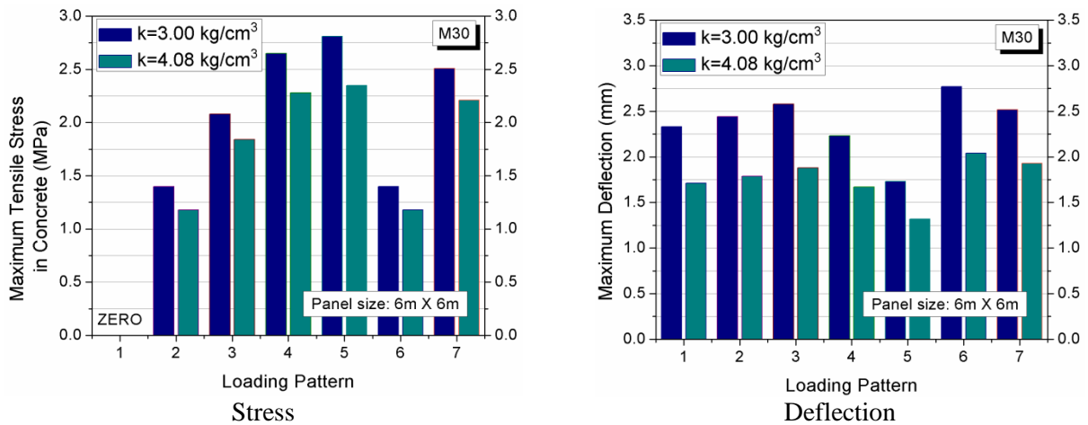
Fig. 3 – Maximum responses for different loading patterns and modulus of sub-grade reaction
