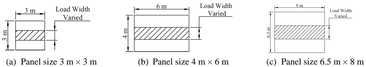
Fig. 4 – Variation of the loading width in loading pattern 5 for identification of the critical loading width for various panel sizes
