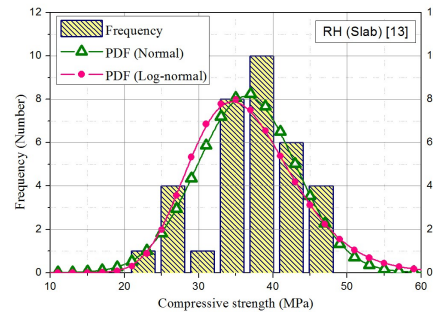
Fig.5 – Compressive strength from RH for slab [14]
