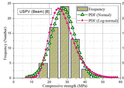
Fig.7 – Compressive strength from USPV for beam [7]
