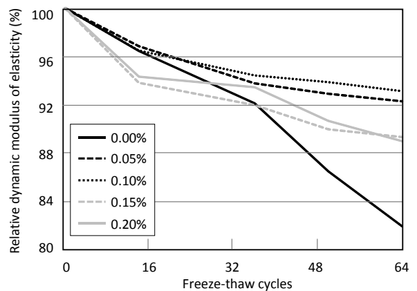
Fig. 7 – Changes in relative dynamic modulus of elasticity of Group B specimens
