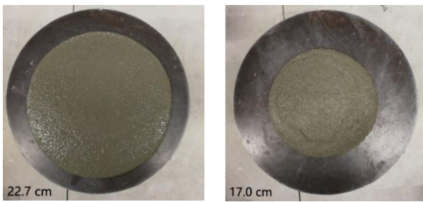
(a) Plain mortar (b) Mortar with 0.2 vol.% basalt fibers
