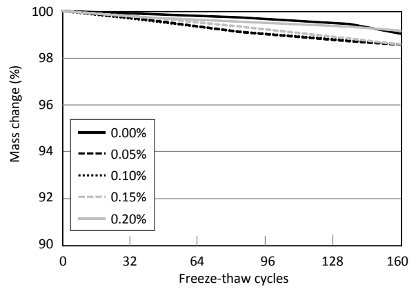
Fig. 4 – Changes in mass of Group A specimen
