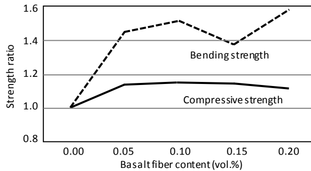
Fig. 10 – Strength ratios after 160 freeze-thaw cycles
