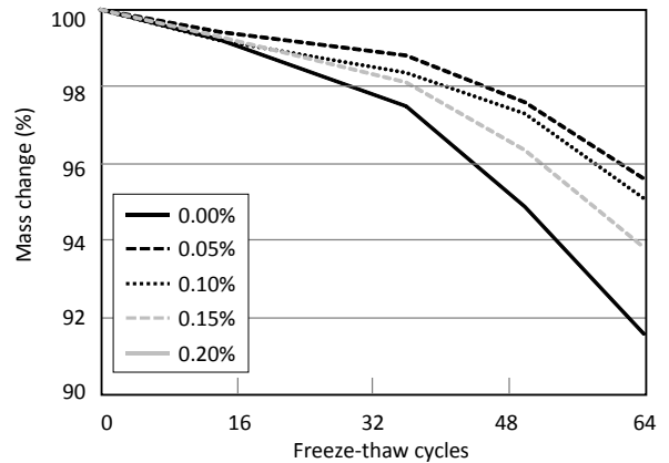
Fig. 5 – Changes in mass of Group B specimens
