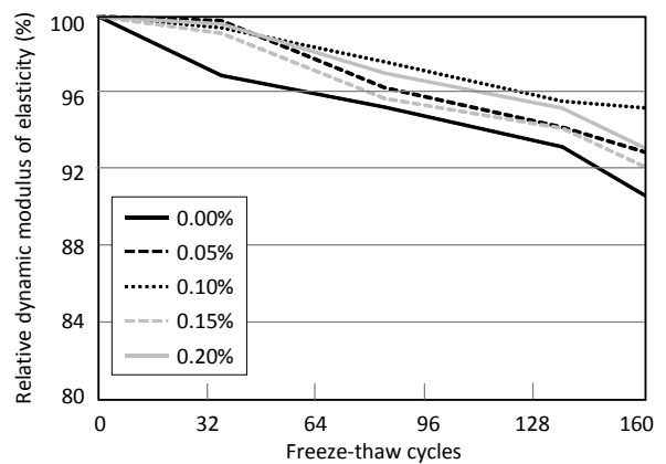
Fig. 6 – Changes in relative dynamic modulus of elasticity of Group A specimens
