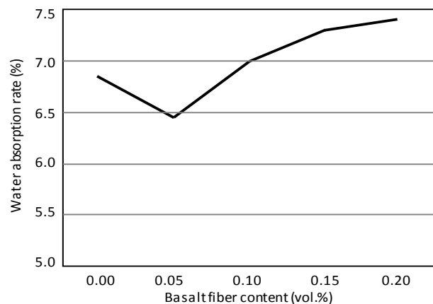
Fig. 11 – Water absorption rate
