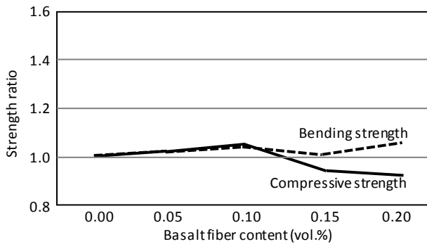
Fig. 9 – Strength ratios prior to freeze-thaw cycles
