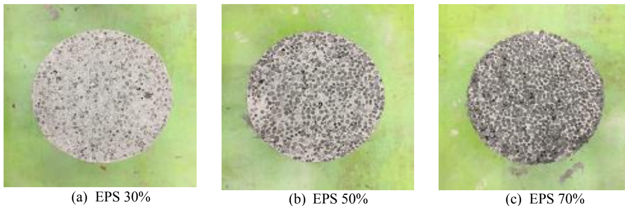
Fig. 1 – Section of UHPEPC specimens depending on the EPS by volume ratio
