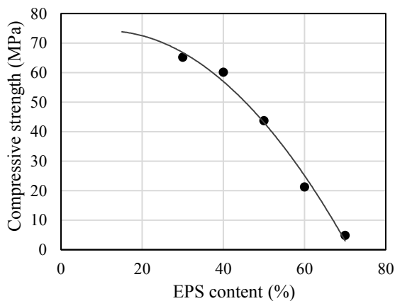
Fig. 2 – Relationship between compressive strength and EPS content by volume ratio
