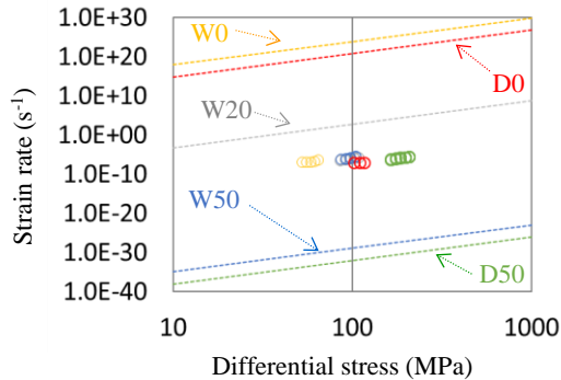
(b) V = 6 \times 10^{-3} \text{ m}^3/\text{mol}
