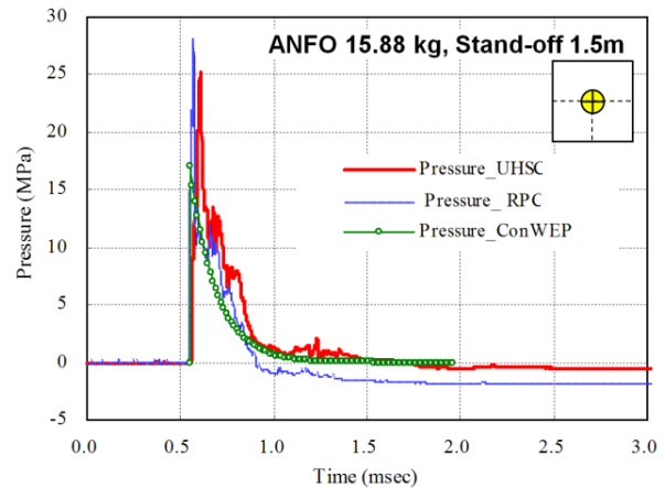
Fig. 7 – Reflected pressures versus time measurements at the center from the main test (15.88 kg ANFO)
