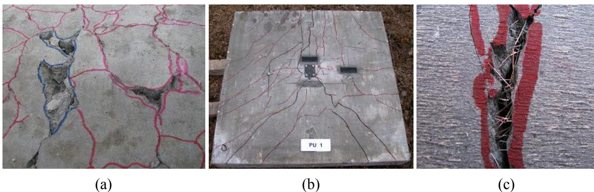
Fig. 6 – Photos of bottom surface of the blasted specimens: (a) NSC, (b) UHSC, (c) RPC
