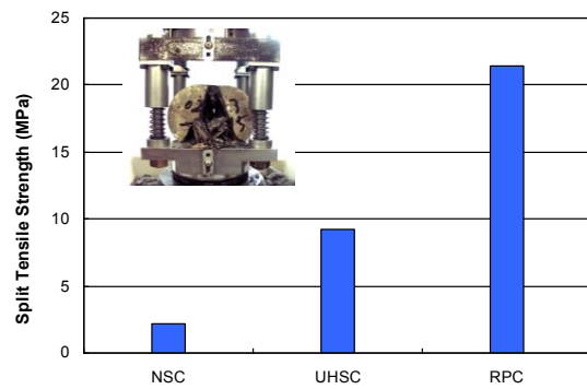
Fig. 2 – Split tensile strength of NSC, UHSC, and RPC
