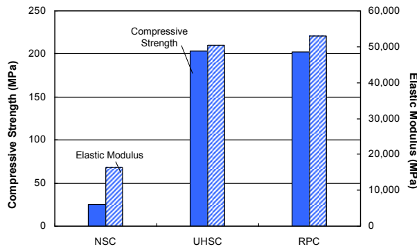
Fig. 1 – Average compressive strength and elastic modulus of NSC, UHSC, and RPC
