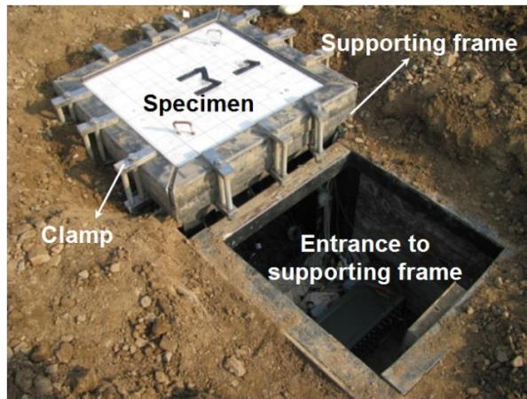
Fig. 3 – Configuration photo of buried supporting frame
