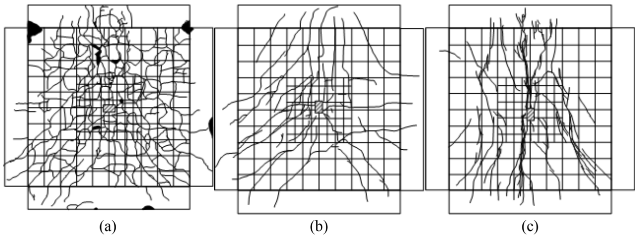
Fig. 5 – Bottom surface crack patterns of blasted specimens: (a) NSC (b) UHSC (c) RPC
