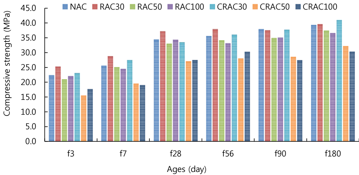
Fig. 4 – Compressive strength test results by age
