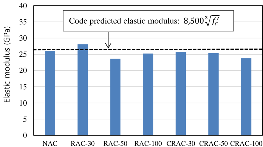
Fig. 7 – Elastic modulus at 28 days
