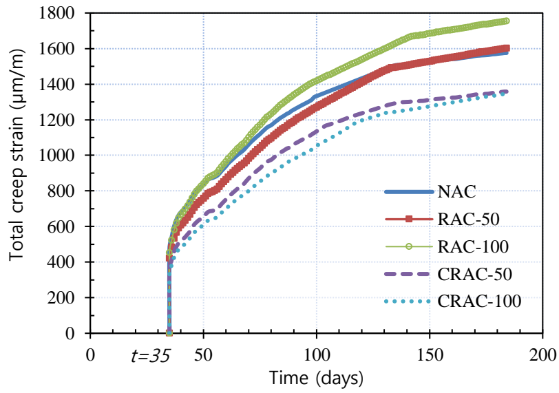
Fig. 11 – Total strain vs. time
