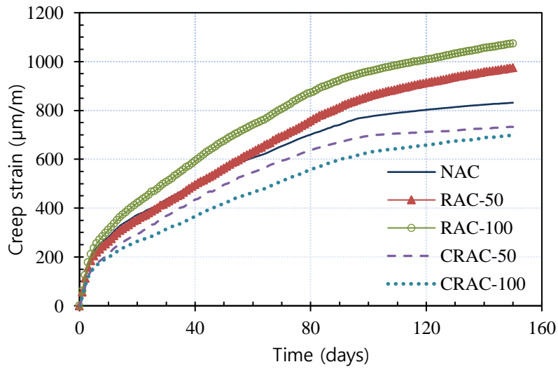
Fig. 12 – Creep vs. time after loading
