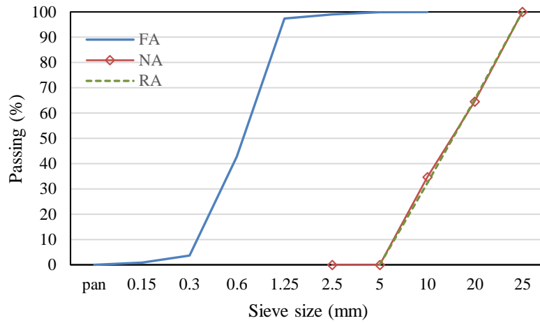
Fig. 1 – Gradation of NA, RA and FA
