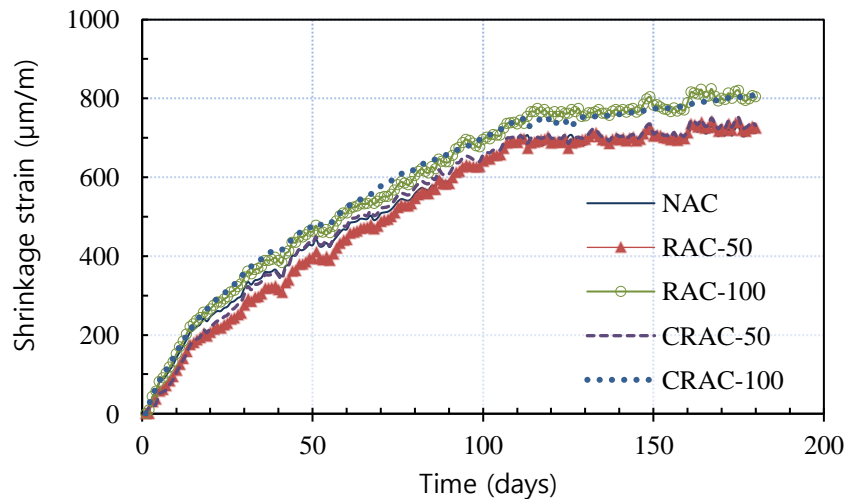
Fig. 9 – Shrinkage vs. time
