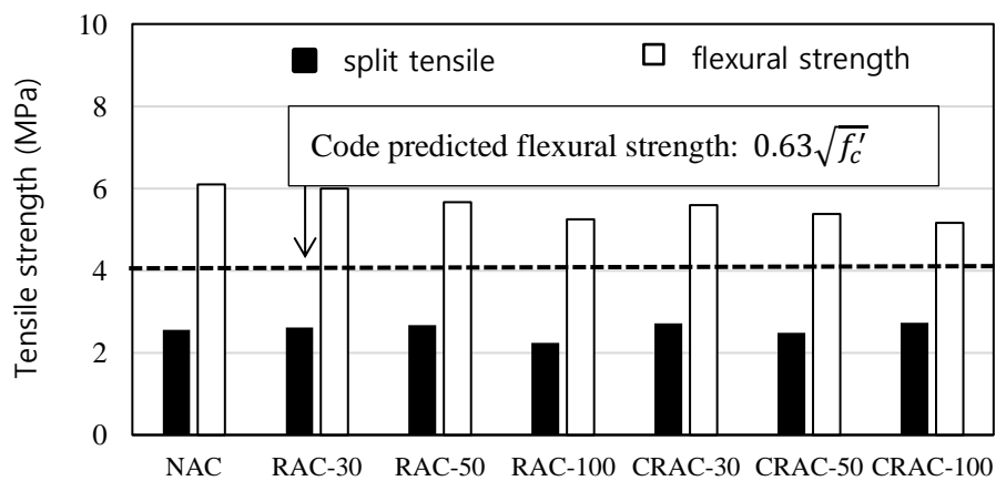
Fig. 6 – Tensile strength at 28 days
