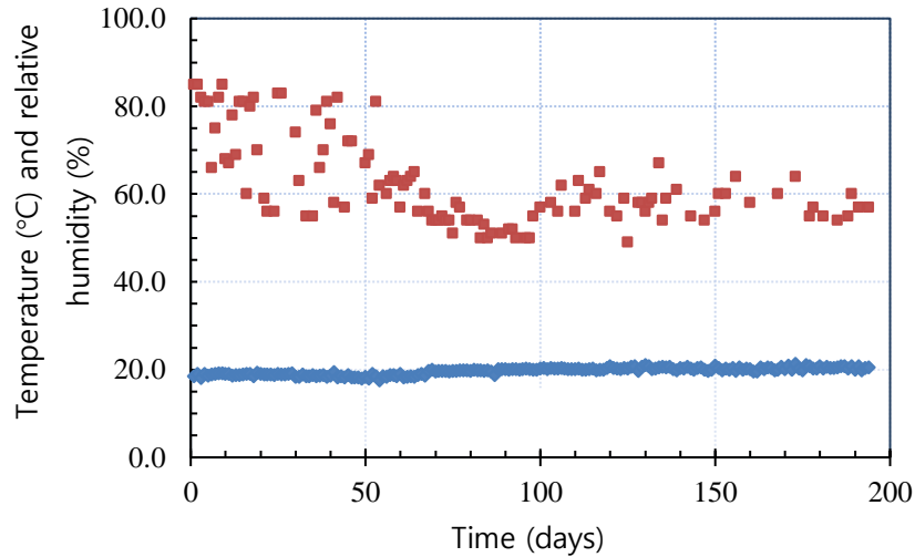
Fig. 8 – Temperature and R.H. in environmental chamber
