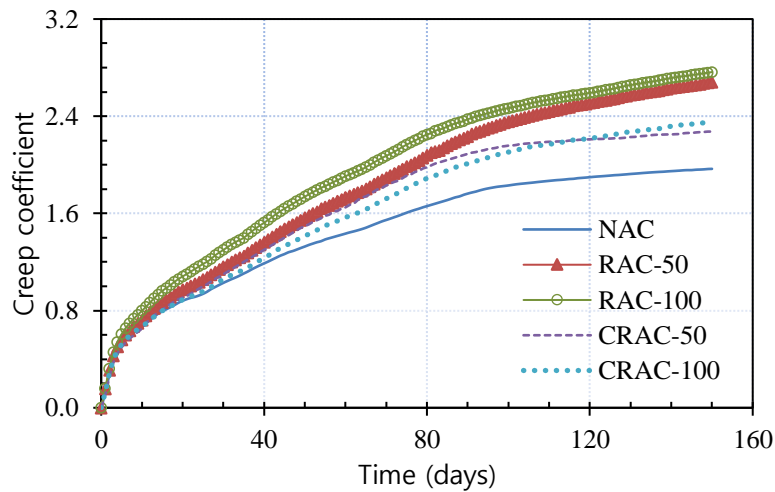
Fig. 14 – Creep coefficients vs. time after loading
