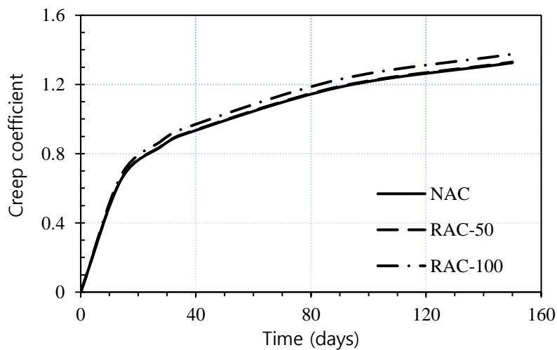
Fig. 15 – Creep coefficient prediction model by ACI 209 [29]
