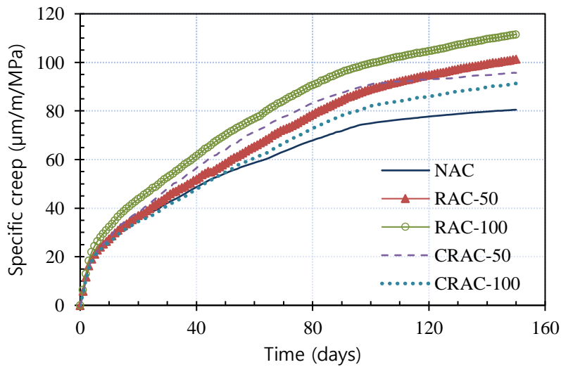
Fig. 13 – Specific creep vs. time after loading
