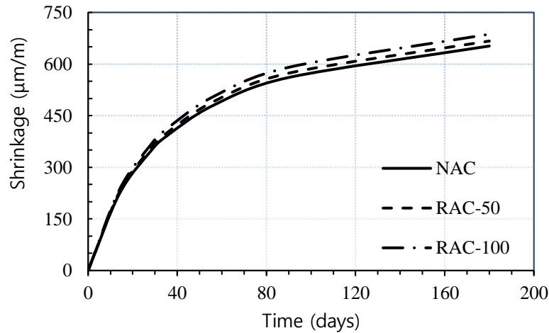
Fig. 10 – Shrinkage prediction model by ACI 209 [29]
